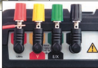
Terminal Adapters are optional accessories used to allow the DET3 and DET4 Series units' terminals to accept alternative cable connections.
