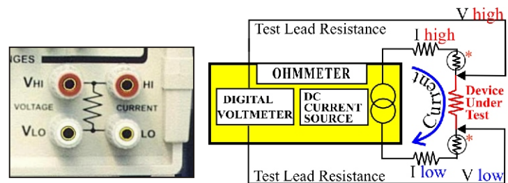
* connection contact resistance
